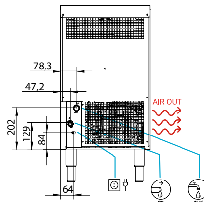
REAR VIEW VISTA POSTERIORE
