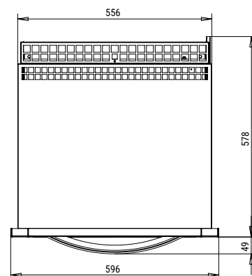
FLOOR VIEW VISTA PLANTA
