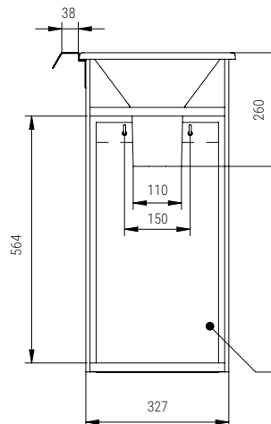
FRONTAL VIEW VISTA FRONTALE
