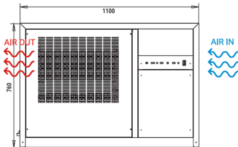
FRONTAL VIEW VISTA FRONTAL
