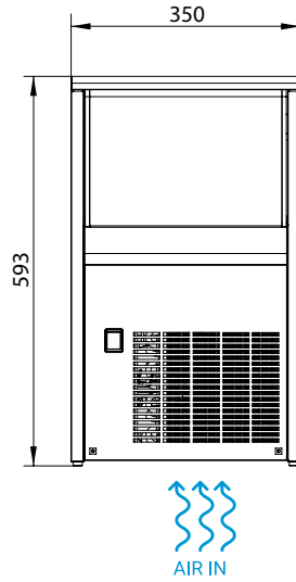
FRONTAL VIEW VISTA FRONTALE
