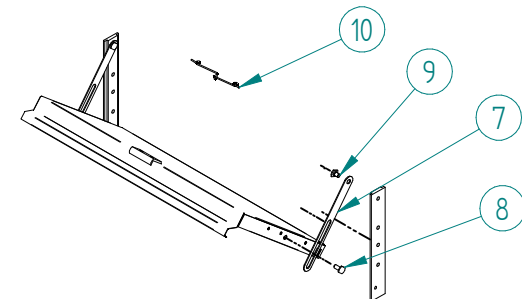
Door variant P25-35
