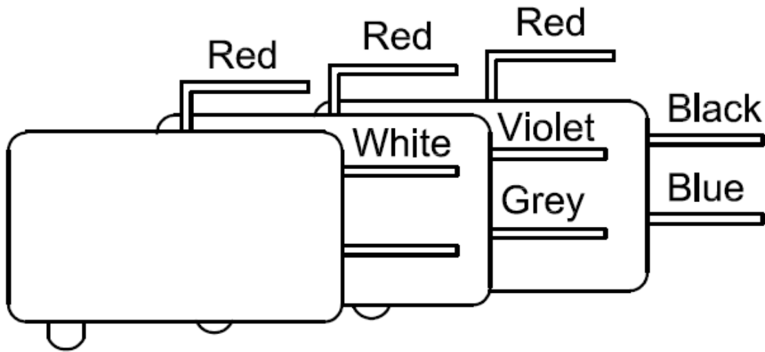
Micro-switch connection CDC timer (grey)
